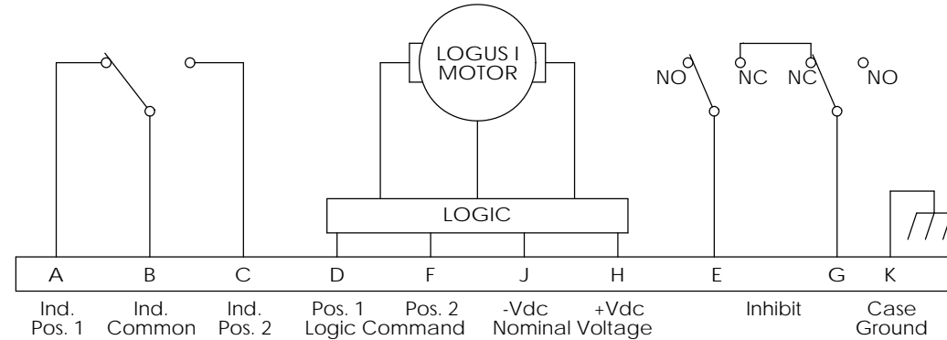
LATCHING, TTL, INHIBIT CLOSED DURING SWITCHING, SHOWN IN POSITION 1
