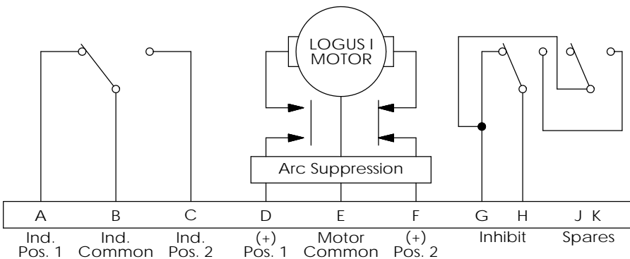
LATCHING, INHIBIT OPEN DURING SWITCHING, SHOWN IN POSITION 1
