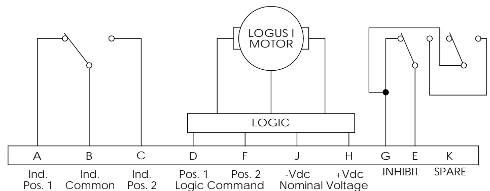
LATCHING, TTL, INHIBIT OPEN DURING SWITCHING, SHOWN IN POSITION 1
