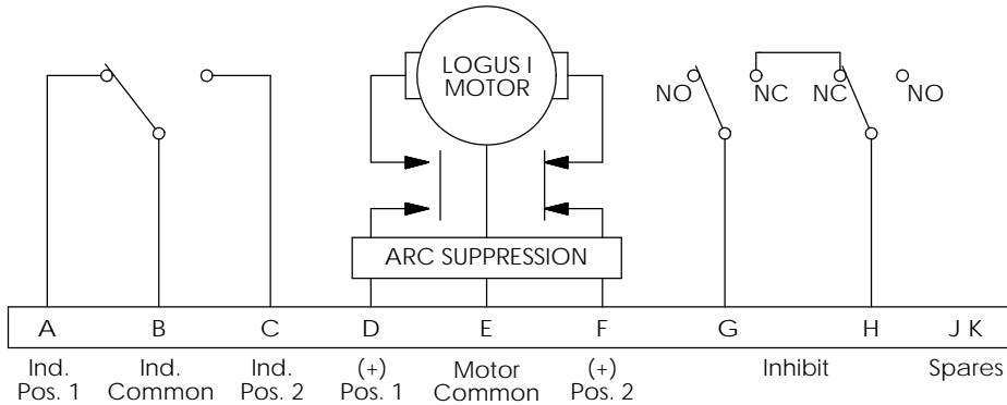
LATCHING, INHIBIT CLOSED DURING SWITCHING, SHOWN IN POSITION 1
