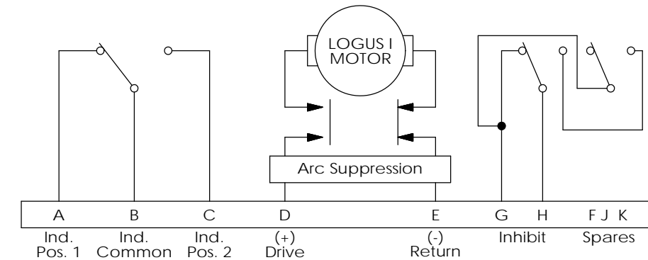
FAILSAFE, INHIBIT OPEN DURING SWITCHING, SHOWN IN POSITION 1, DE-ENERGIZED
