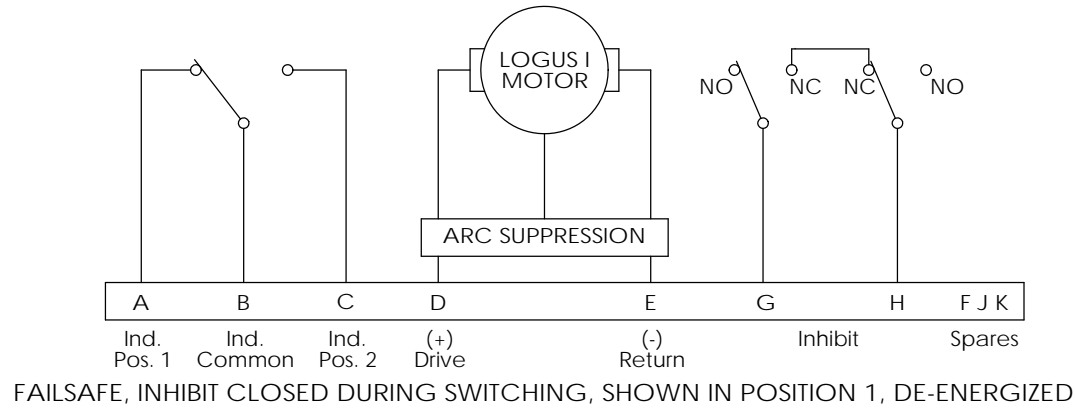
Electrical Circuit E, Connector MS3112E-12-10P
