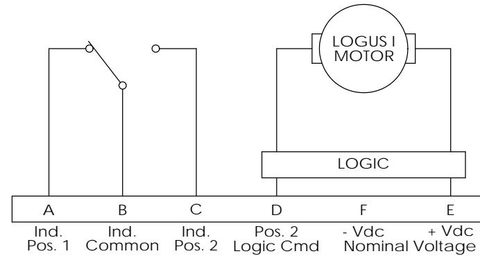
FAILSAFE, SHOWN IN POSITION 1
