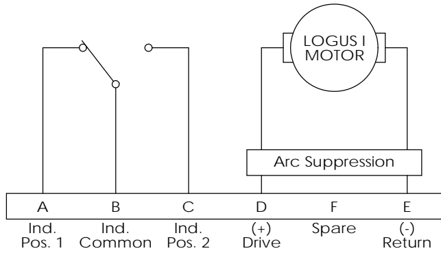
FAILSAFE, SHOWN IN POSITION 1
