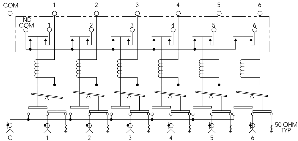
SCHEMATIC DIAGRAM SHOWN IN NORMALLY OPEN POSITION (DE-ENERGIZED)
