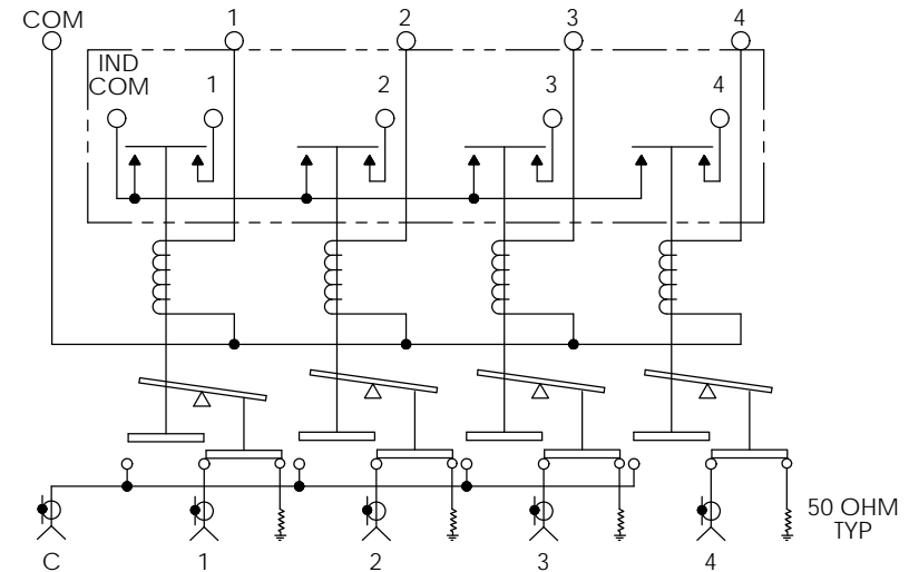
SCHMATIC DIAGRAM SHOWN IN NORMALLY OPEN POSITION (DE-ENERGIZED)
