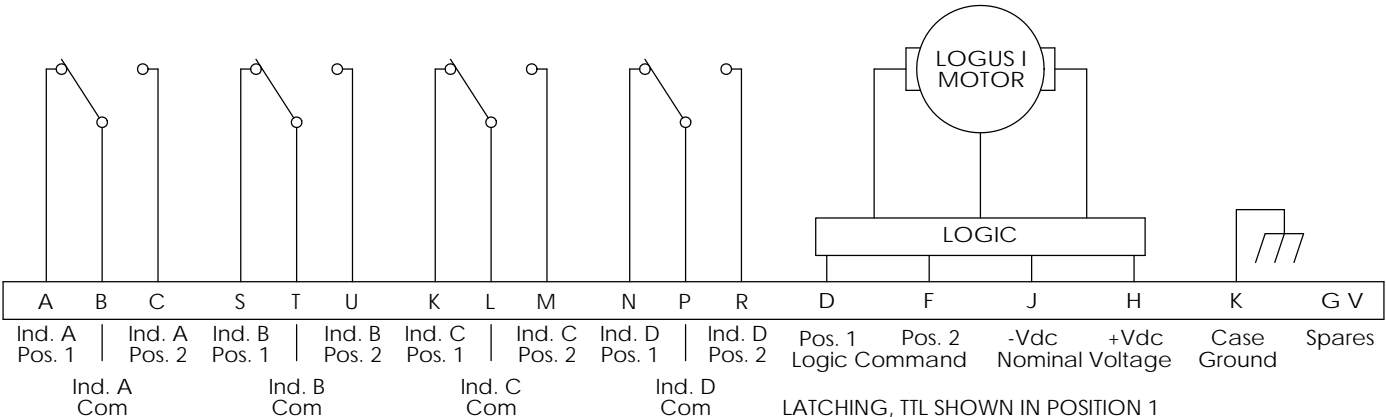
Electrical Circuit D w/TTL, Connector MS3112E-14-19P
