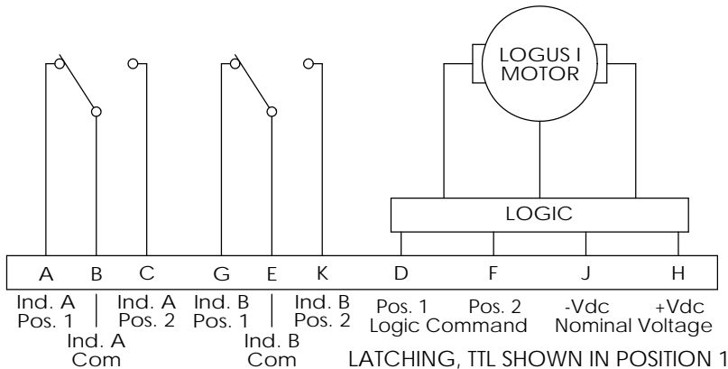
Electrical Circuit B w/TTL, Connector MS3112E-12-10P
