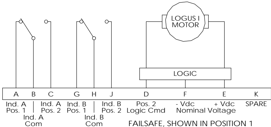
Electrical Circuit B, w/TTL, Connector MS3112E-12-10P
