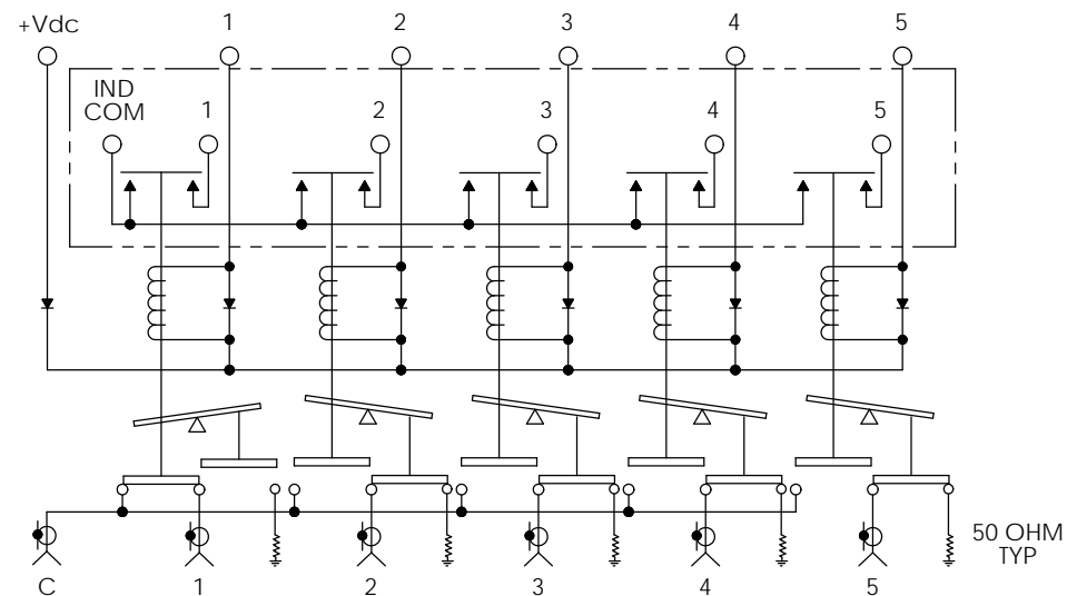
SCHEMATIC DIAGRAM SHOWN IN POSITION 1
