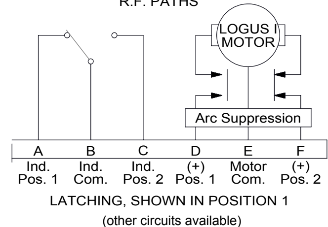
R.F. PATHS
